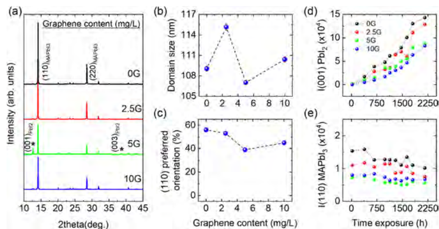
Figure 1. (a) XRPD profiles ( \text{Cu K}\alpha 1/\alpha 2 ) of the 0G–10G \text{MAPbI}_3 films at 300 K. The asterisks indicate the impurity of \text{PbI}_2 . (b) Variation of the average crystal domain size of the \text{MAPbI}_3 films with the graphene content. (c) Preferred orientation–graphene concentration relationship of the \text{MAPbI}_3 films. Time evolution of (d) (001) reflection intensity of the \text{PbI}_2 degradation product and (e) (110) reflection intensity of \text{MAPbI}_3 .
