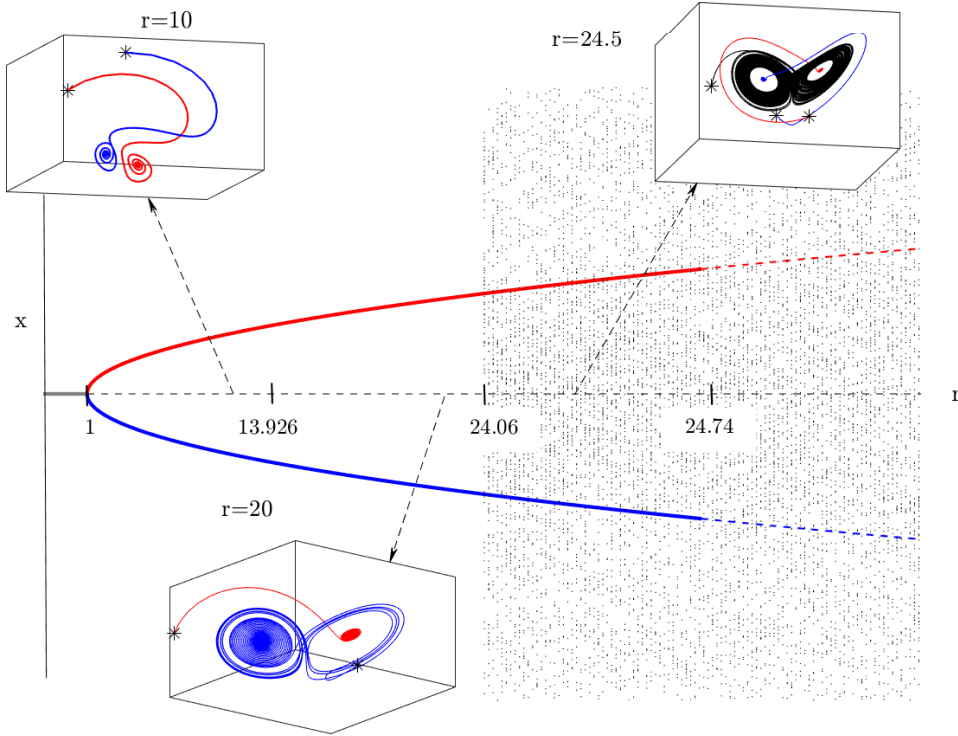
Fig. 1. Bifurcation diagram for the Lorenz system. For r = 1 a supercritical pitchfork bifurcation takes place and the origin becomes a saddle point. For 1 < r < 24.06 , two attractors coexist: the upper branch corresponds to C^+ and the lower branch corresponds to C^- . For this range of r values, past the homoclinic bifurcation (when r > 13.926 ), trajectories may be chaotic before settling to one of the two fixed point attractors. For r > 24.06 , the chaotic attractor is born in a heteroclinic bifurcation and the three attractors coexist. Finally, for r > 24.74 a subcritical Hopf bifurcation leaves the chaotic attractor as the global attractor. In the insets, the attractors are represented in phase space for the regions where multistability is present (the stars mark the initial conditions).
