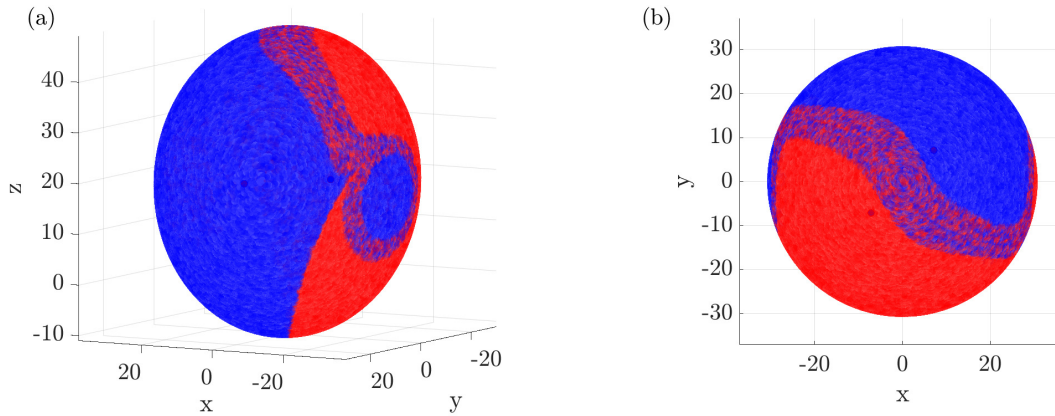
Fig. 2. Basins of attraction for r = 20 . (a) The sphere of initial conditions is represented with the trajectories that end up in the C^+ attractor depicted in red and the ones that end up in C^- depicted in blue. The attractors are also represented in the inside as points with matching colors. (b) We present a view in the (x, y) plane. Fractality appears in the basin boundaries for z > (r - 1) = 19 .
