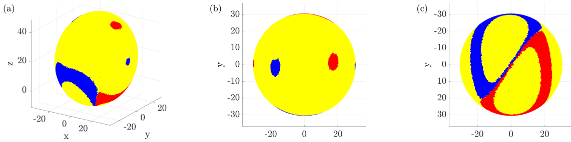
Fig. 4. Basins of attraction for r = 24.5 . (a) The sphere of initial conditions is represented with the same color code as before: red accounts for C^+ and blue for C^- . Yellow regions account for trajectories that head to the chaotic attractor. The (b) and (c) panels show the (x, y) plane for z > 19 (view from above) and z < 19 (view from the downside) respectively.
