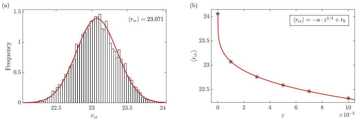
Fig. 7. Critical value of the parameter r and scaling law for the heteroclinic dynamic bifurcation. (a) The normal distribution of r_{cr} for an ensemble of trajectories with a specific rate of change of \varepsilon = 10^{-3} . (b) The mean value of r_{cr} for different values of \varepsilon . The stars correspond to numerically calculated values of \langle r_{cr} \rangle , the power law fit is also shown in red.
