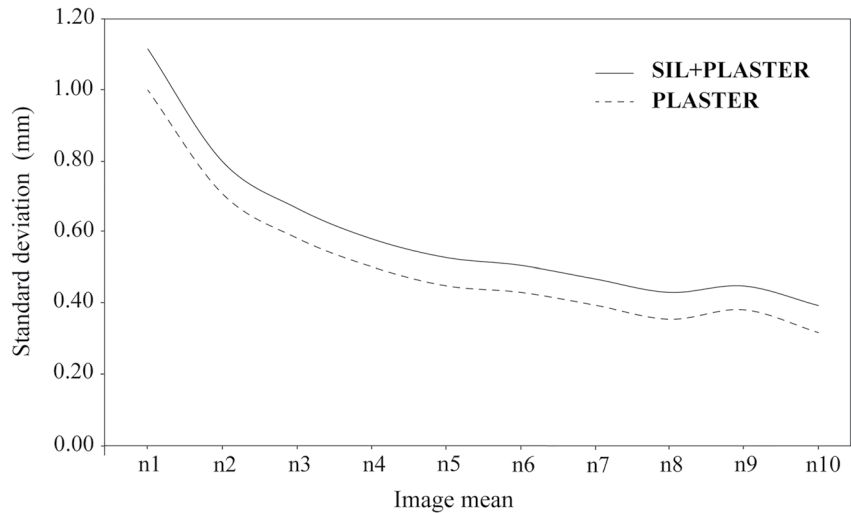
Figure 5. Variation of the standard deviation value obtained by averaging with different number of images for two different materials (PLASTER and SIL + PLASTER). Note that at both cases the main reduction of standard deviation value occurs for the averaging involving up to five images (n5).
