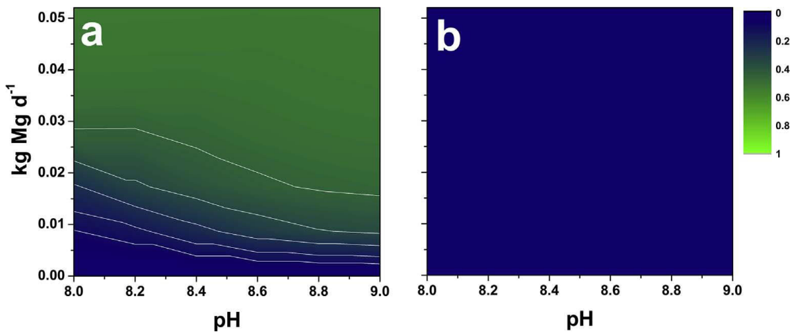
Figure 4. Model based evaluation of the potential P recovery in the form of struvite as a fraction of the total load entering the system for AD1 (a) and AD2 (b). The legend indicates normalized phosphorus recovery
