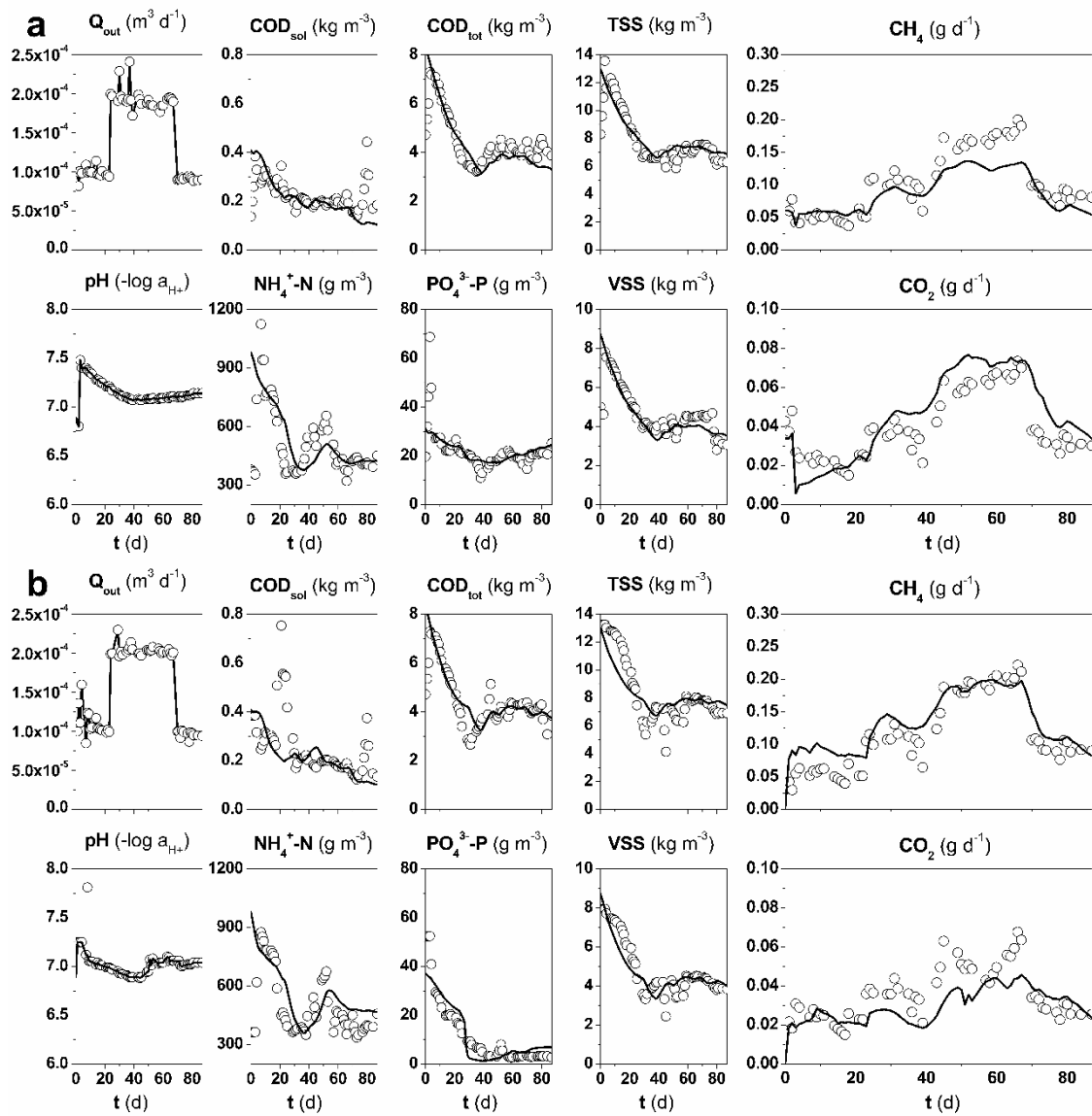
Figure 2. Experimental results (open symbols) and simulation data (continuous lines) for AD1 (a) and AD2 (b). Note that graph titles correspond to Y axes labels for improving data visualization.
