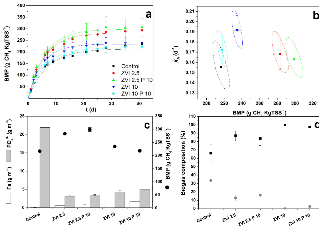
Figure 1. Results of biochemical methane potential assays. Experimental (symbols) and first order-modeled (lines) methane production (a); 95% confidence regions for k_H and BMP values (b); and dissolved Fe and \text{PO}_4^{3-} compared to methane production (c) and biogas composition: \text{CH}_4 (squares) and \text{CO}_2 (circles) (d) at the end of the experiments. Error bars are 95% confidence intervals. ZVI concentrations are in \text{kg Fe m}^{-3} . P 10 indicates that 10 \text{ g PO}_4^{3-}\text{-P m}^{-3} were added at the beginning of the experiment.
