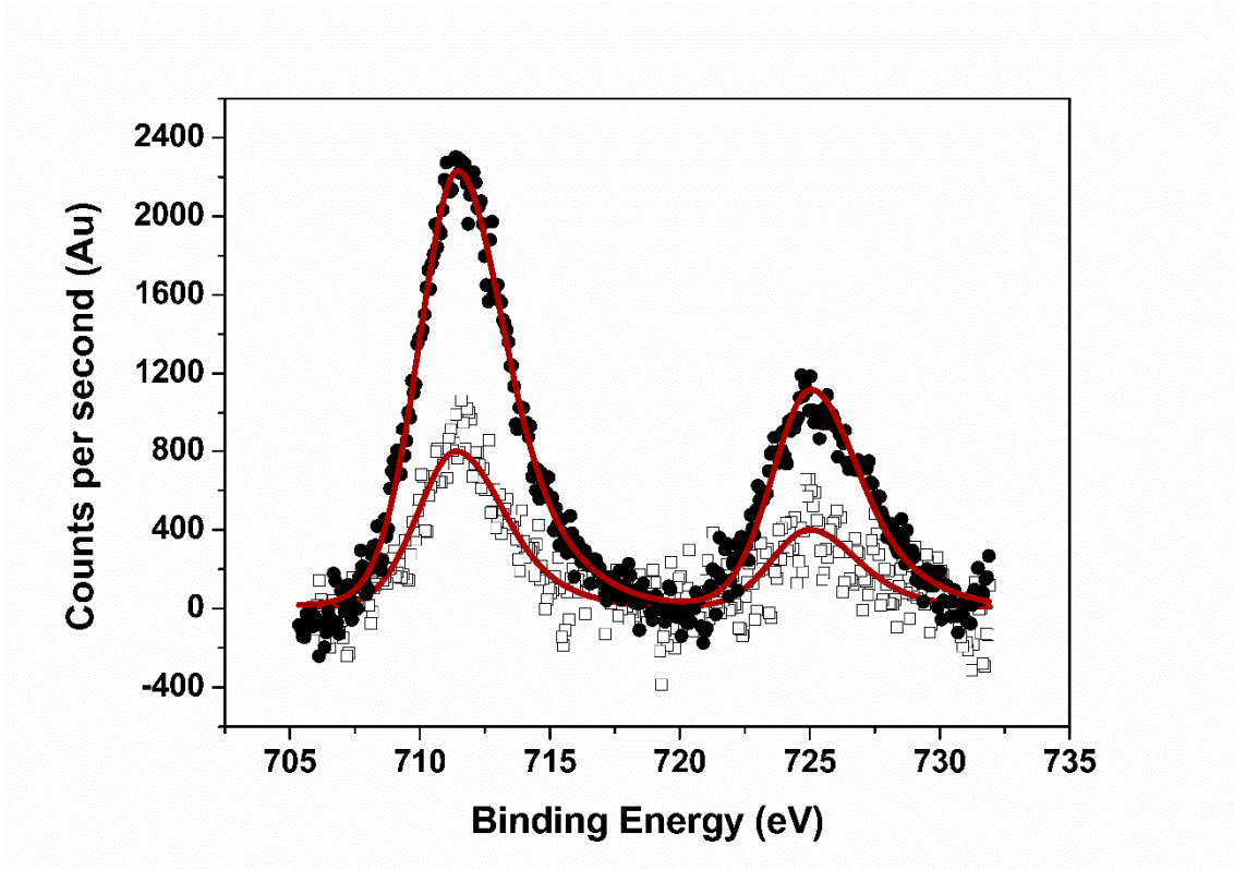
Figure 3: Fe2p core-level spectra of AD1 (squares) and AD2 (circles) outlet samples in stage 3.
