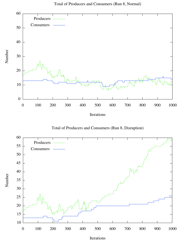
Figure 7: Sample runs of category 3, total number of producer and consumers, normal conditions (top figure); disrupted conditions (bottom figure). Normal run does not exhibit regular growth pattern and instead stagnates or even declines, but is stabilized after the disruption into a consistent growth pattern.
