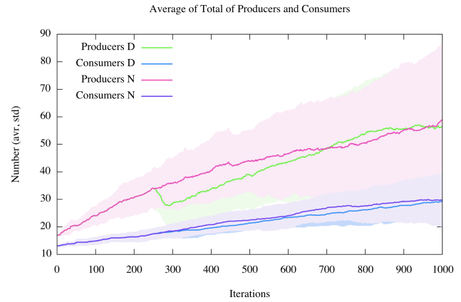
Figure 4: Mean number (lines) and standard deviation (shaded areas) of producer and consumer agents for 15 unperturbed normal (N) and perturbed or disrupted (D) runs. Color shades are indicating 1 standard deviation for each class of runs.
