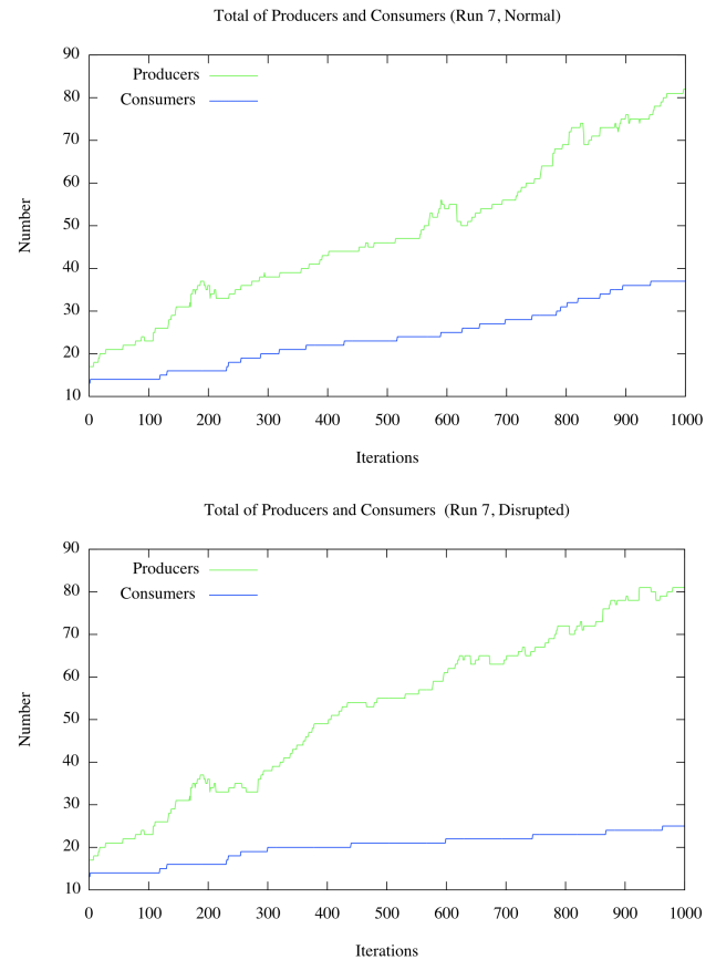
Figure 5: Sample runs of category 1, total number of producer and consumers, normal conditions (top figure); disrupted conditions (bottom figure). Both runs exhibit growth behaviour.
