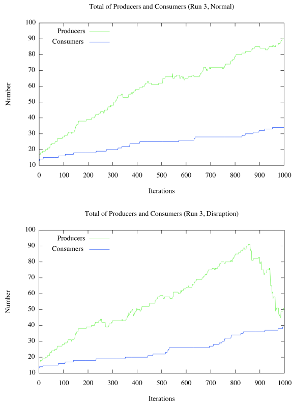
Figure 6: Sample runs of category 2, total number of producer and consumers, normal conditions (top figure); disrupted conditions (bottom figure). Major decline in disrupted system after a long delay.
