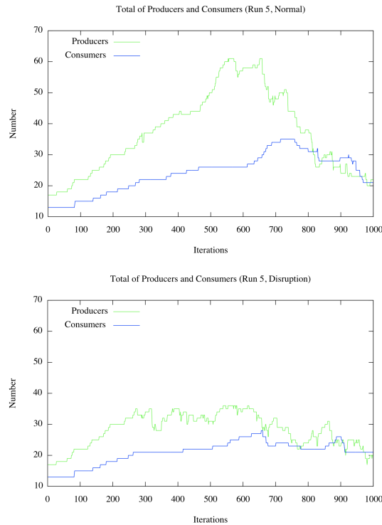
Figure 8: Sample runs of category 4, total number of producer and consumers, normal conditions (top figure); disrupted conditions (bottom figure). Both normal and disrupted runs do not exhibit regular growth patterns.
