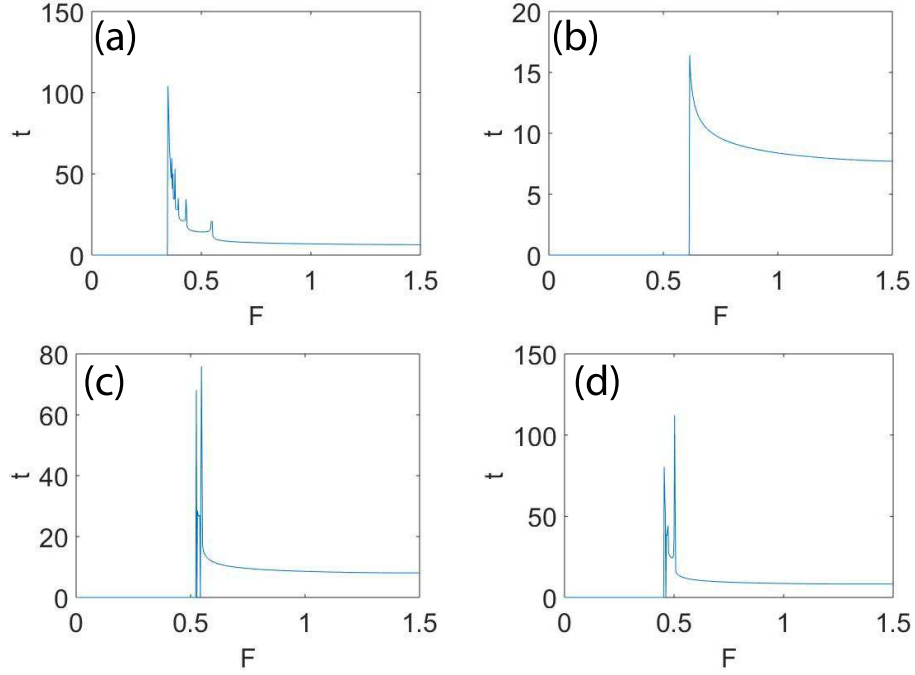
FIG. 14: The panel shows the particle escape times from the potential well with \alpha = 0.25, 1, 1.25, 1.39 , by reading the figures from (a) to (d), and varying F .
