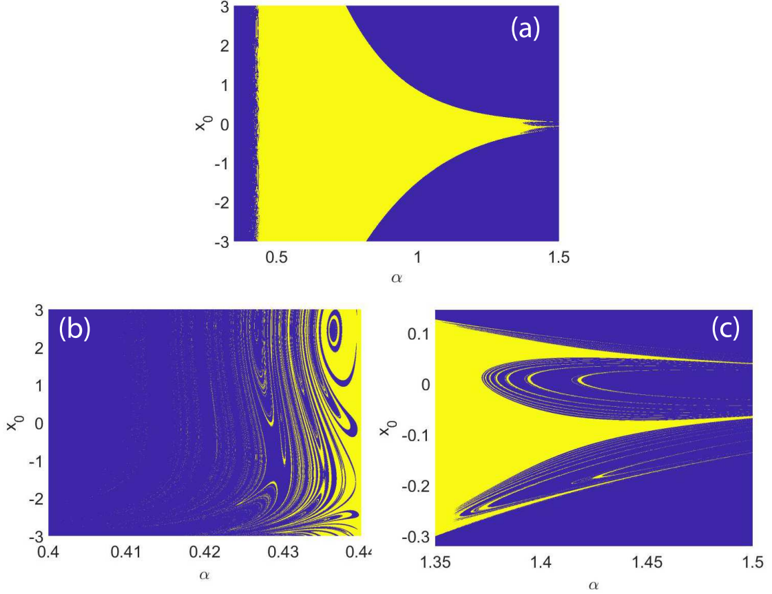
FIG. 7: Final state of the system depending on the \alpha -value and the variation of the first initial condition x_0 from -3 to 3 . White color (yellow on line) implies the particle remains inside the well and black color (blue on line) that particle escapes. In figure (a) We can see in this figure a defined area representing the last state of the particle as time goes on depending on the initial position x_0 and on the \alpha variation, keeping constant the rest of the parameters of the model. In figures (b) and (c) it is possible to appreciate the zoom of the figure (a) for values of \alpha = (0.4, 0.44) and \alpha = (1.35, 1.5) , respectively. These last ones are the areas where the boundaries show the fractalization.
