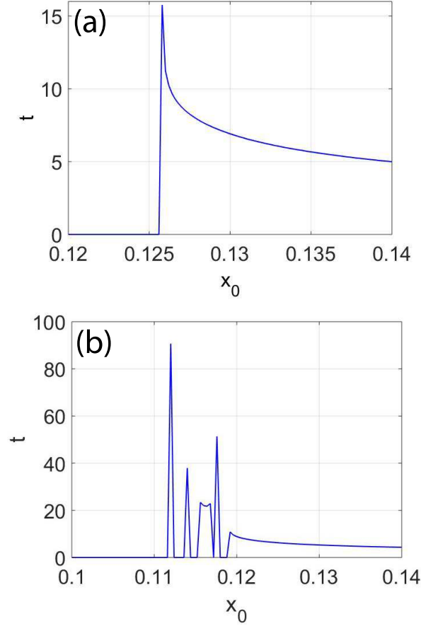
FIG. 10: (a) Average escape times from the well for \alpha = 1.35 and different initial conditions inside the well. (b) The same for \alpha = 1.36 . It is possible to observe that from values of \alpha \approx 1.36 the escape times, before to show the monotonic decay, have fluctuations.
