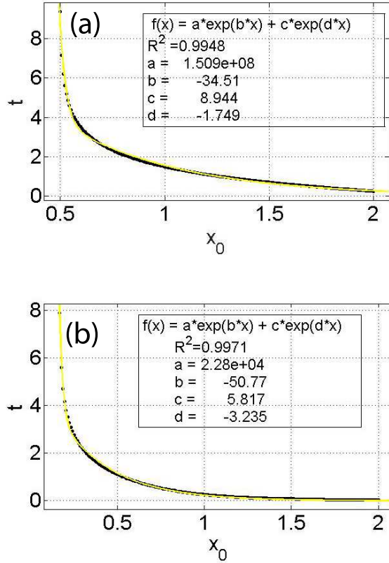
FIG. 9: (a) Average escape times from the well for \alpha = 1.1 versus different initial conditions inside the well. (b) Represents the same for \alpha = 1.3 . It is possible to observe the exponential decay law.
