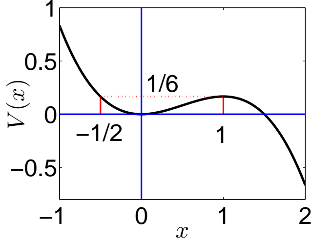
FIG. 1: Plot of the potential well defined through the function V(x) = \frac{1}{2}x^2 - \frac{1}{3}x^3 . Note that for the interval x \in [-\frac{1}{2}, 1) in absence of forcing and friction the orbits are bounded.
