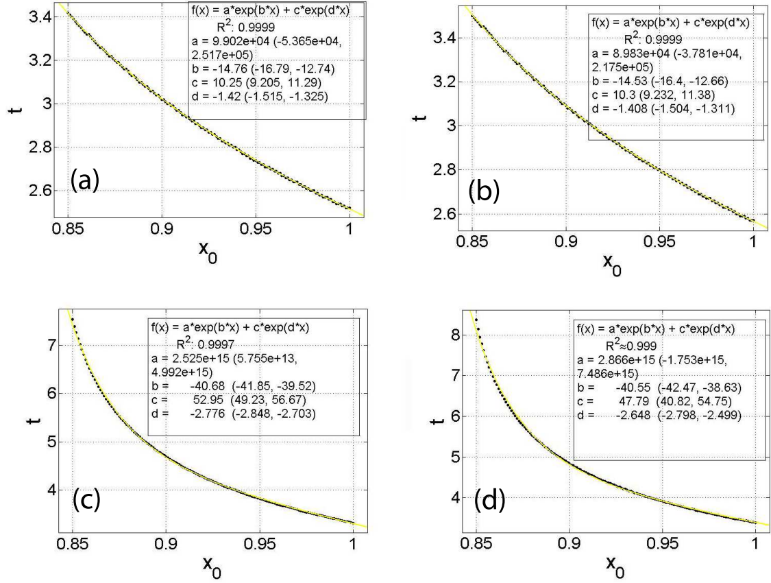
FIG. 3: Comparison between escape times of solutions provided by distinct methods for the damped Helmholtz oscillator at x_0 \in (0.85, 1) with \mu = 0.1 in panels (a) and (b), \mu = 0.8 in panels (c) and (d). In all the panels F = 0.46 and \omega = 1 . Panels (a) and (c) show the escape times calculated with the Runge-Kutta method. Panels (b) and (d) show the escape times calculated with the fractional numerical scheme and \alpha = 1 . In the textboxes we can see the fitting equations and their parameter. Near the parameter, in the parenthesis, we show the 95% confidence bounds. This is important to check that the fitting equations and their parameters values of each couple of panels, (a)-(b) and (c)-(d), are compatible within each other.
