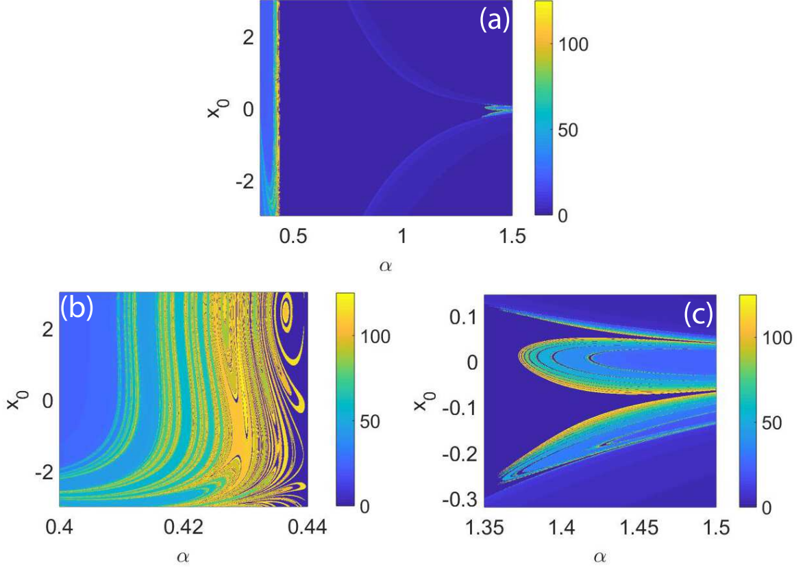
FIG. 8: Figure (a) shows the gradient of the particle escape times from the potential well depending on the variation of the \alpha value and of the first initial condition x_0 from -3 to 3 . Figures (b) and (c) present a zoom of the most interesting areas of figure (a), i.e., values of \alpha = (0.4, 0.44) and \alpha = (1.35, 1.5) , respectively. As stated in the previous panel, the areas where the boundaries show the fractalization.
