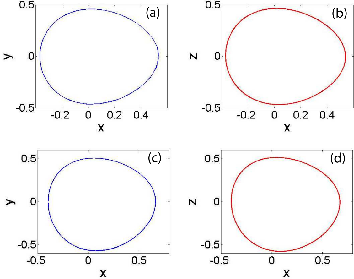
FIG. 2: Comparison between solutions provided by distinct methods for the damped Helmholtz oscillator at the zero initial conditions with \mu = 0.1 and F = 0.1 in panels (a) and (b), \mu = 0.8 and F = 0.46 in panels (c) and (d). Panels (a) and (c) show the trajectories of the solution of the fourth-order Runge-Kutta scheme. Panels (b) and (d) show the trajectories of the solution of the fractional numerical scheme with \alpha = 1 .
