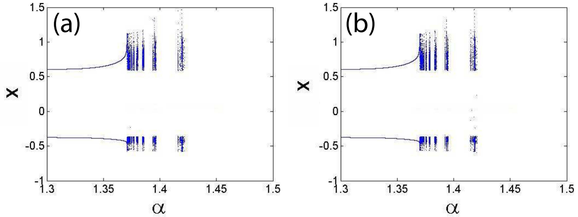
FIG. 16: Bifurcation diagram with x_0 = 0.0 , \mu = 0.8 , F = 0.46 and \omega = 1 (a). Bifurcation diagram with x_0 = 0.01 , \mu = 0.8 , F = 0.46 and \omega = 1 (b)
