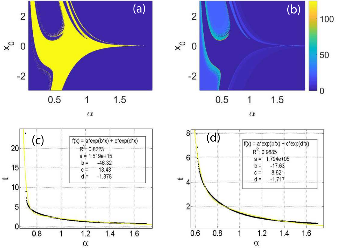
FIG. 4: Figure (a) shows the final state of the system depending on the value of \alpha , from 0.1 to 2, and the variation of the first initial condition x_0 from -3 to 3 . White color (yellow on line) implies that the particle remains inside the well and black color (blue on line) that particle escapes. In (a) it is possible to see the areas where the boundaries show the fractalization. Figure (b) shows the gradient of the particle escape times from the potential well depending on the \alpha -value and the variation of the first initial condition for the same values of figure (a). Figures (c) and (d) show an example of the trend of the escape time in function of \alpha , for different initial conditions, x_0 = -2 and x_0 = -3 respectively.
