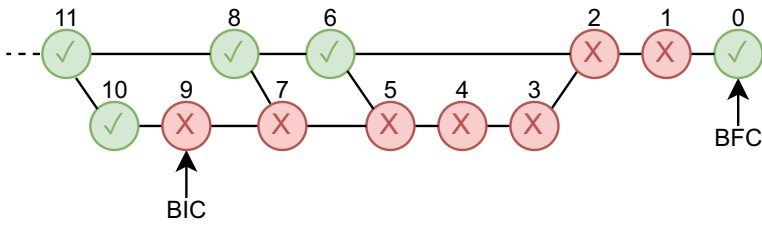
Fig. 2 Visual representation of the results of the experiment for Bug 41 of JacksonDataBind project
