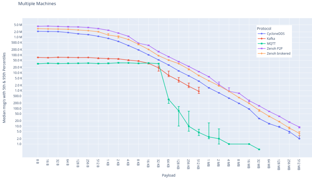
Figura 3.8: Rendimiento de distintos protocolos [Eclipse and ZettaScale, 2023]
