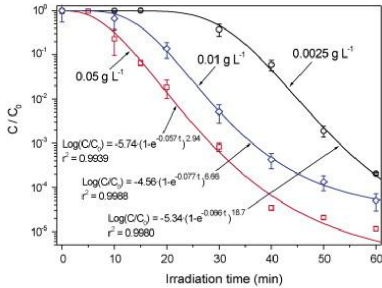
Fig. 3. Fitting of the modified Hom kinetic model to experimental data of the photocatalytic inactivation of 10^6 CFU mL ^{-1} E. coli suspensions with different loadings of Degussa P25 TiO _2 (error bars calculated from eight independent bacteria counting measurements).
