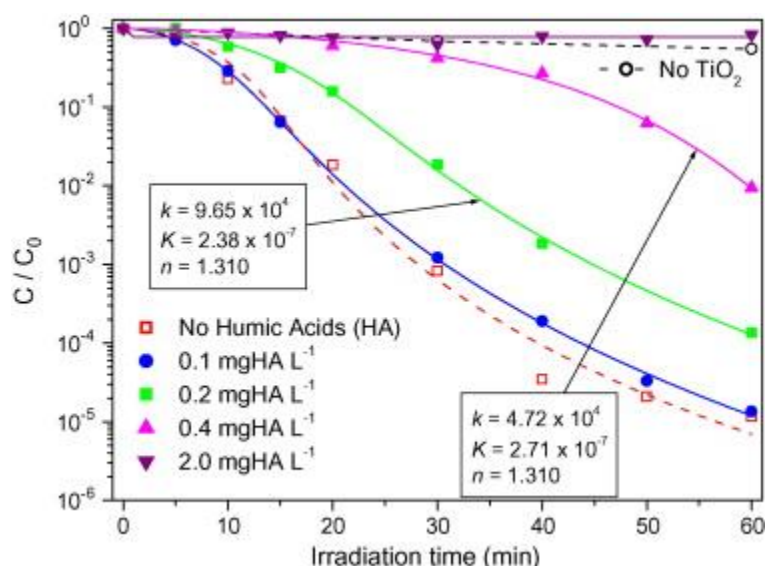
Fig. 12. Influence of the humic acids concentration on the photocatalytic inactivation of 10^6 CFU mL -1 E. coli suspensions with 0.05 \text{ g L}^{-1} of Degussa P25 TiO 2 (error bars have been omitted for clarity purposes). Lines show the fitting of the experimental data with the kinetic model represented by eqs. (16) and (17). Units of k : CFU mL -1 min -1 ; units of K : mL n CFU - n ; n dimensionless.
