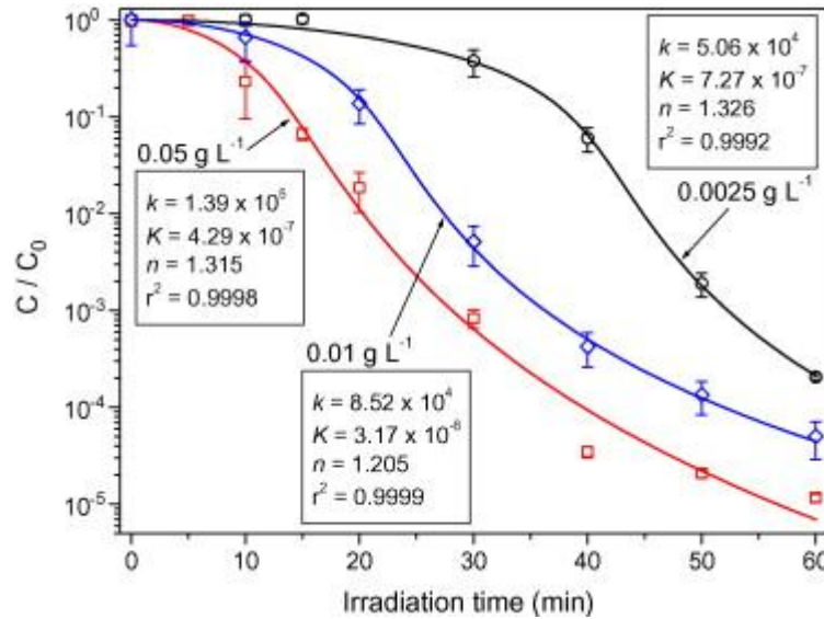
Fig. 4. Fitting of the kinetic model to experimental data of the photocatalytic inactivation of 10^6 CFU \text{mL}^{-1} E. coli suspensions with different loadings of Degussa P25 \text{TiO}_2 (error bars calculated from eight independent bacteria counting measurements). Units of k : \text{CFU mL}^{-1} \text{min}^{-1} ; units of K : \text{mL}^n \text{CFU}^{-n} ; n dimensionless.
