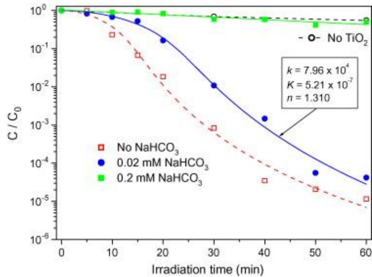
Fig. 10. Influence of the bicarbonate concentration on the photocatalytic inactivation of 10^6 \text{CFU mL}^{-1} E. coli suspensions with 0.05 \text{ g L}^{-1} of Degussa P25 \text{TiO}_2 (error bars have been omitted for clarity purposes). Lines show the fitting of the experimental data with the kinetic model represented by eqs. (16) and (17). Units of k : \text{CFU mL}^{-1} \text{ min}^{-1} ; units of K : \text{mL}^n \text{ CFU}^{-n} ; n dimensionless.
