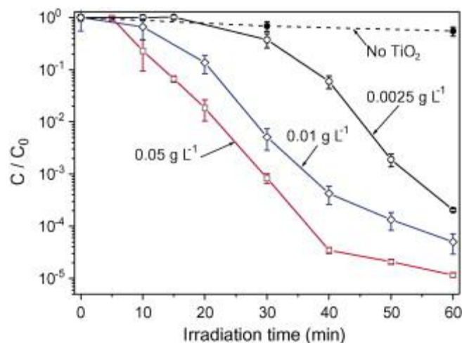
Fig. 1. Photocatalytic inactivation of 10 6 CFU mL -1 E. coli suspensions with different loadings of Degussa P25 TiO 2 (error bars calculated from eight independent bacteria counting measurements).
