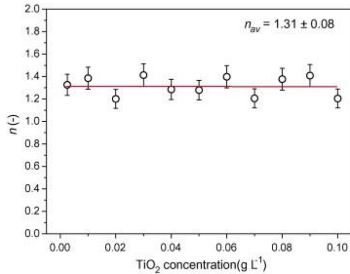
Fig. 7. Influence of Degussa P25 TiO 2 loading on the inhibition coefficient for the photocatalytic inactivation of 10 6 CFU mL -1 E. coli suspensions (error bars calculated from two independent experiments).
