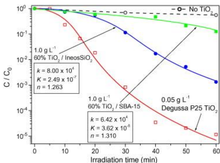
Fig. 8. Photocatalytic inactivation of 10^6 CFU mL -1 E. coli suspensions with two different silica-supported TiO 2 photocatalysts (error bars have been omitted for clarity purposes). Lines show the fitting of the experimental data with the kinetic model represented by eqs. (16) and (17). Units of k : CFU mL -1 min -1 ; units of K : mL n CFU - n ; n dimensionless.
