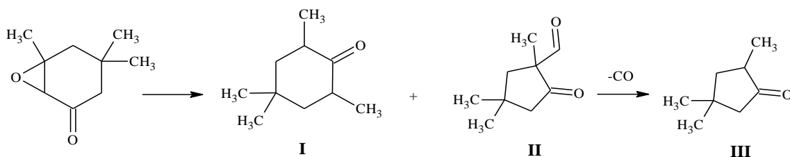
Scheme 4. Products obtained in isomerisation of isophorone oxide: 3,5,5-trimethyl-1,2-cyclohexanedione (I) and 2-formyl-2,4,4-trimethylcyclopentanone (II) and subsequent deformylation of (II) to 2,4,4-trimethylcyclopentanone (III).
