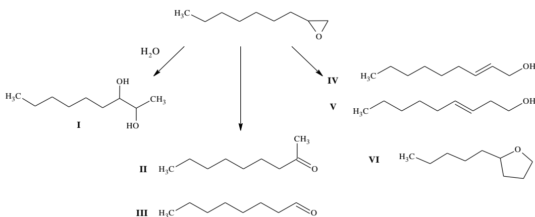
Scheme 3. Products obtained in isomerisation of 1,2 epoxyoctane: 1,2-octanediol (I), 2-octanone (II), octanal (III), 2-octen-1-ol (IV), 3-octen-1-ol (V) and 2-butyltetrahydrofuran (VI).
