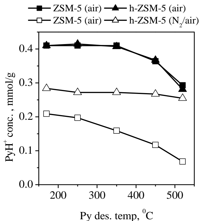
Figure 7. Evolution of the pyridine adsorbed on Brønsted acid sites of the different samples as the evacuation temperature is increased.
