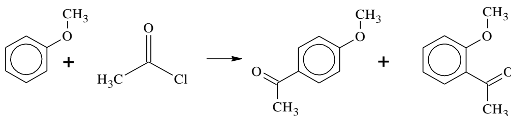
Scheme 1. Anisole acylation.
