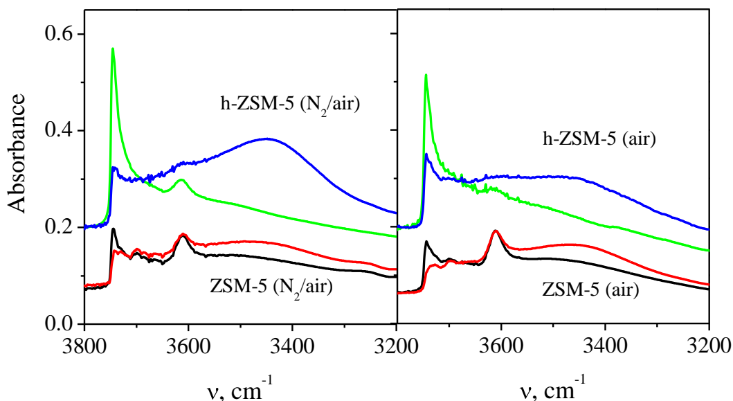
Figure 8 IR spectra of OH groups in ZSM-5 zeolites before and after pivalonitrile adsorption, followed by 5 min evacuation at ambient temperature.
