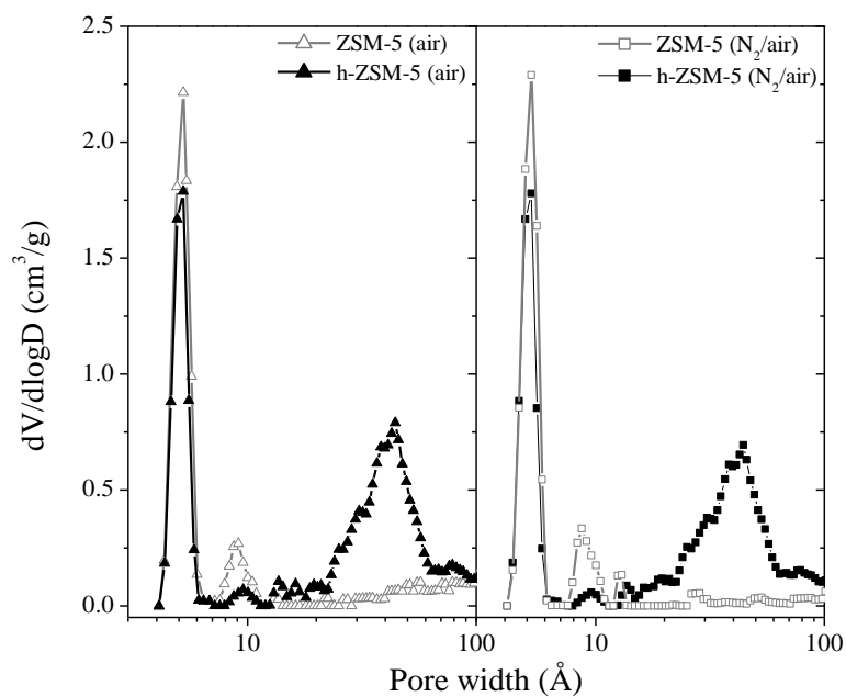
Figure 3. NLDFT pore size distributions of the ZSM-5 samples.
