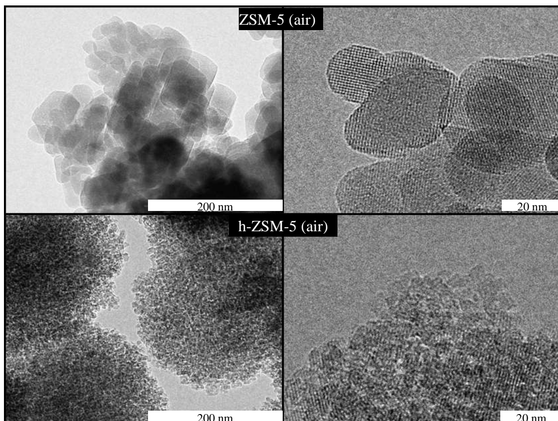
Figure 4. TEM images of ZSM-5 (air) and h-ZSM-5 (air) samples.
