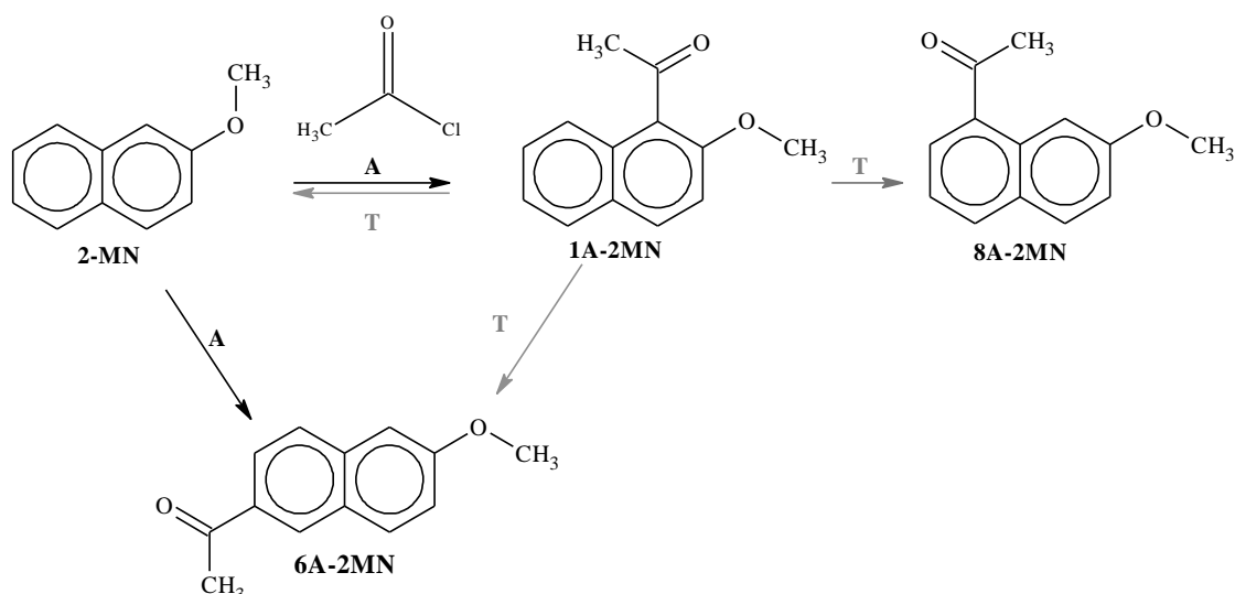
Scheme 2. 2-MN acylation reaction scheme.
