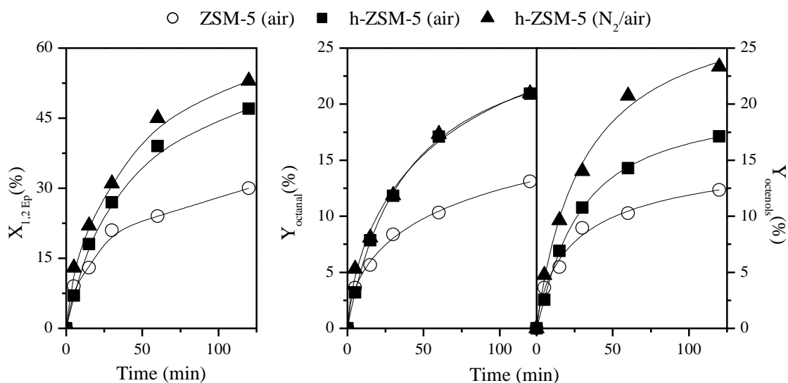
Figure 11. 1,2 epoxyoctane isomerization: conversion (left) and octanal and octenols yield (right).
