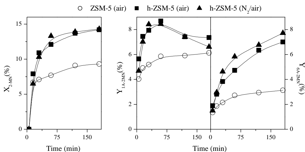
Figure 10. 2-MN acylation: conversion (left) and 1A-2MN and 6A-2MN yields (right).
