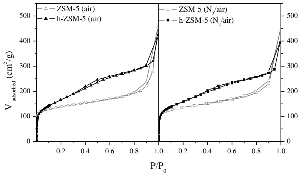
Figure 2. Ar adsorption–desorption isotherms at 87 K of the ZSM-5 samples.
