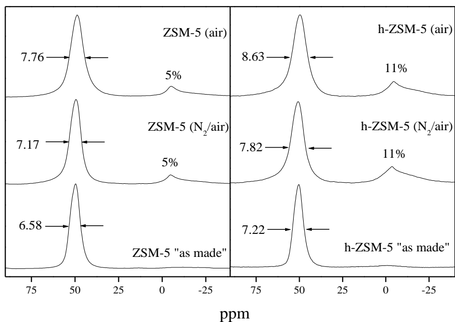
Figure 5. ^{27}\text{Al} MAS NMR spectra of the parent ZSM-5 materials and of samples after different calcination treatments.
