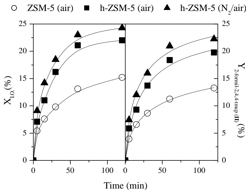
Figure 12. Isophorone oxide isomerization: conversion (left) and 2-formyl-2,4,4-trimethylcyclopentanone yield (right).
