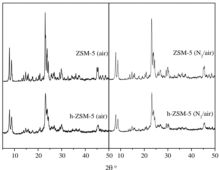
Figure 1. XRD patterns of both hierarchical and standard ZSM-5 samples.
