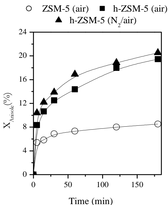
Figure 9. Evolution of the anisole conversion with the reaction time.
