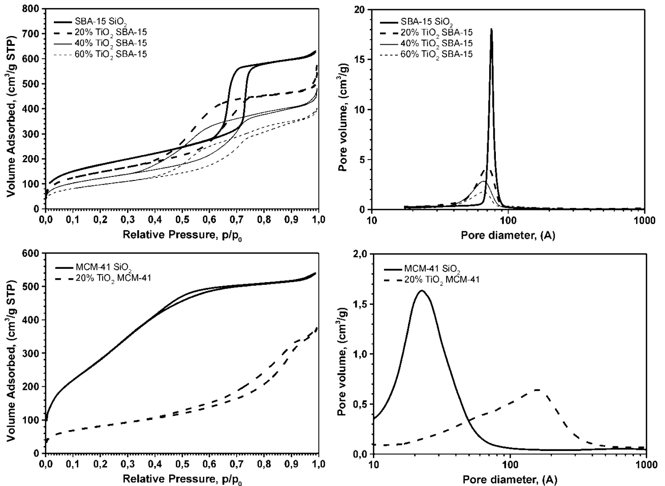
Figure 2. Nitrogen adsorption isotherms of: a) 0 – 60 % TiO 2 _ SBA-15 and b) 0 – 20% TiO 2 _ MCM-41 samples. Pore size distributions of: c) 0 – 60 % TiO 2 _ SBA-15 and d) 0 – 20% TiO 2 _ MCM-41 samples
