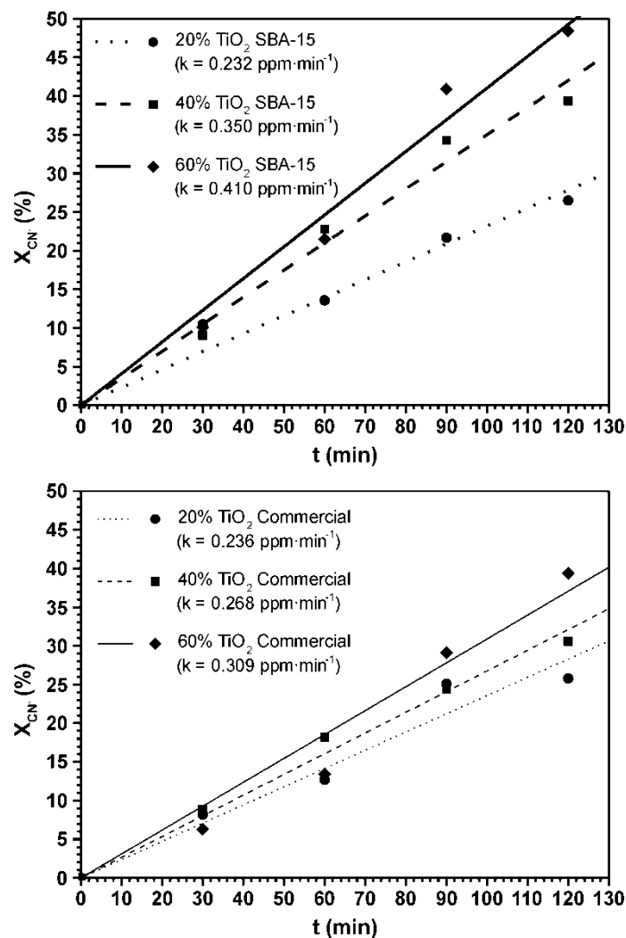
Figure 6. Kinetics of cyanide photooxidation in the presence of: a) 20 – 60% TiO 2 _ SBA-15 samples and b) 20 – 60% TiO 2 _ Commercial SiO 2 materials.
