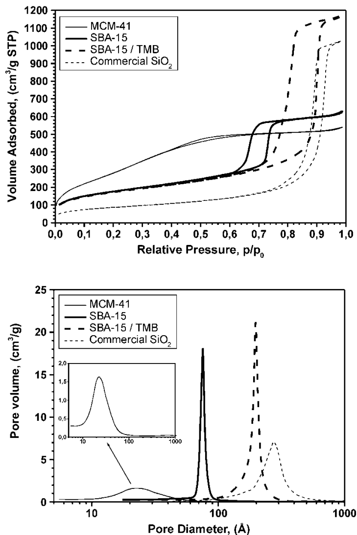
Figure 1. a) Nitrogen adsorption-desorption isotherms and b) pore size distributions of MCM-41, SBA-15, SBA-15/TMB and commercial silica supports.
