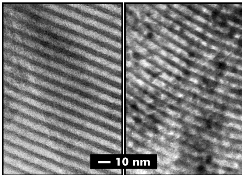
Figure 5. TEM micrographs of: a) SBA-15 and b) 60% TiO 2 -SBA-15 samples.
