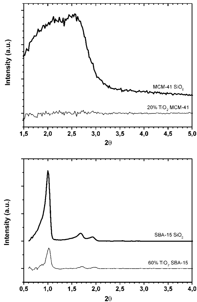
Figure 3. XRD patterns at low angle of: a) MCM-41 and 20% \text{TiO}_2 _ MCM-41 samples and b) SBA-15 and 60% \text{TiO}_2 _ SBA-15 samples.
