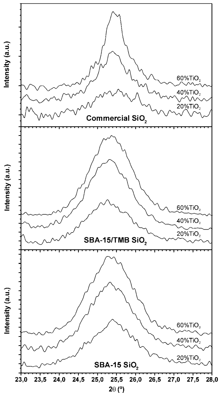
Figure 4. XRD patterns of \text{TiO}_2 supported on: a) commercial silica; b) SBA-15/TMB; and c) SBA-15 silica. Increasing titania loadings in the range 20 wt% to 60 wt% are shown for each support.
