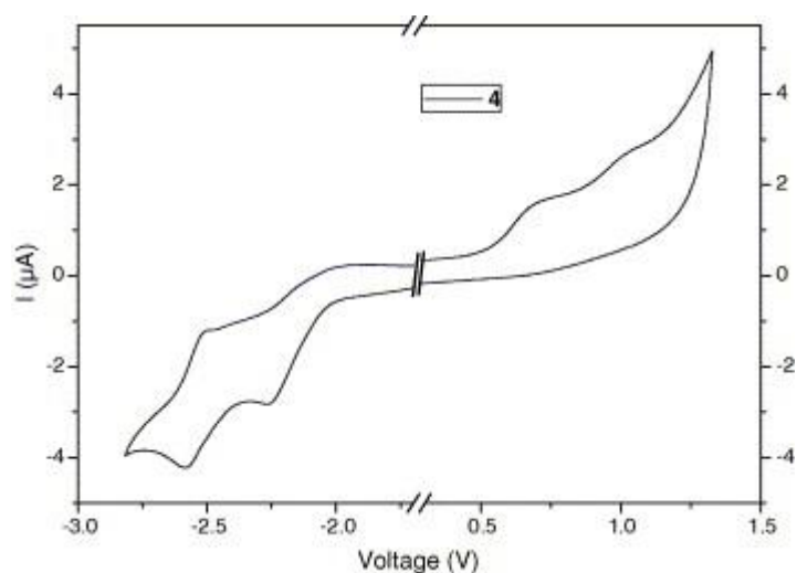
Figure 4. Cyclic voltammogram of 4 in dichloromethane (oxidation) and dimethylformamide (reduction). TBAHFP (0.1 M) solutions, 20 °C, scan rate of 100 mV/s, Pt disk working electrode, potentials versus FC/FC + .
