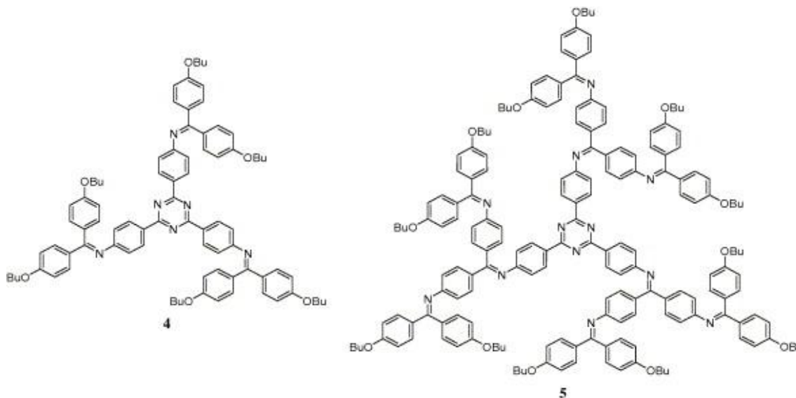
Figure 2. Donor-acceptor dendritic polyphenylazomethines 4 and 5 .
