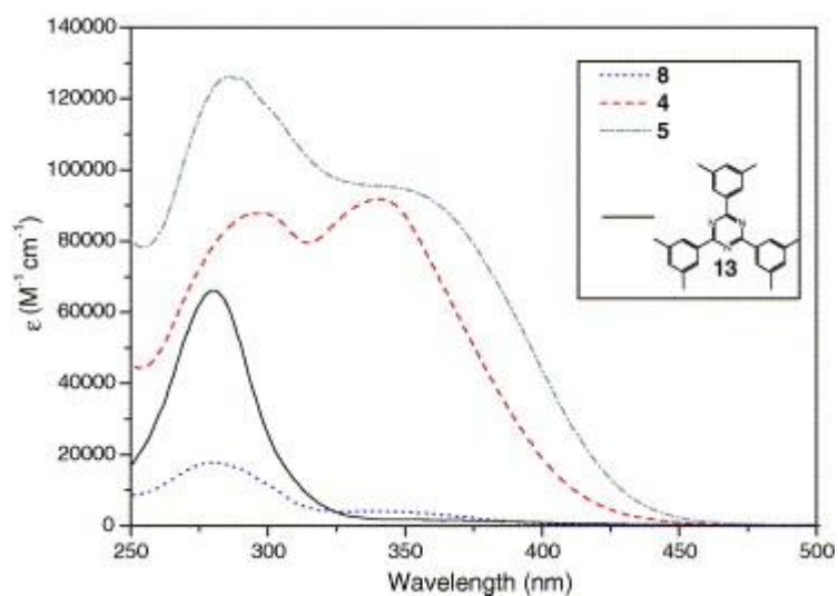
Figure 3. UV–vis absorption spectra of dendrimers 4 and 5, dendron 8 and triazine reference 13 in dichloromethane.
