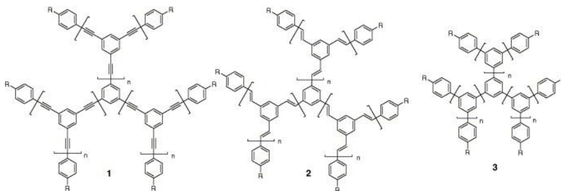
Figure 1. Polyphenyleneethynylene ( 1 ), polyphenylenevinylene ( 2 ) and polyphenylene ( 3 ) type dendrimers.
