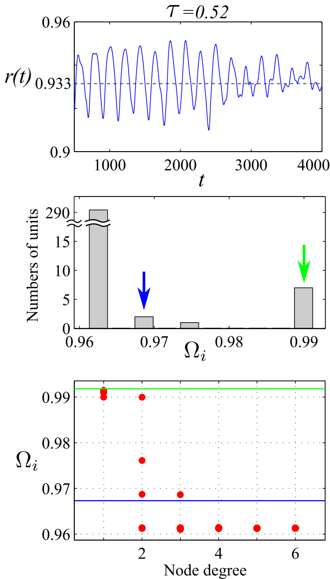
FIG. 3. Time evolution of the synchronization order parameter r(t) with root mean square r = 0.93 (top), histogram over the time averaged frequencies of the oscillators (center), and frequencies versus node degree (bottom) for \tau = 0.52 . In this case Eq. 12 explains the numerical outcome to a good approximation. The values of Eq. 12, for d_i = 1 and d_i = 2 , are marked with arrows in the histogram and solid lines in the bottom figure. The result was obtained from a computer simulation of Eqs. (2) on a network with a binomial degree distribution with 300 nodes. The mean node degree \langle d_i \rangle was equal to 4, other parameters values were K = 0.1 , k = 4 and \omega = 1 .
