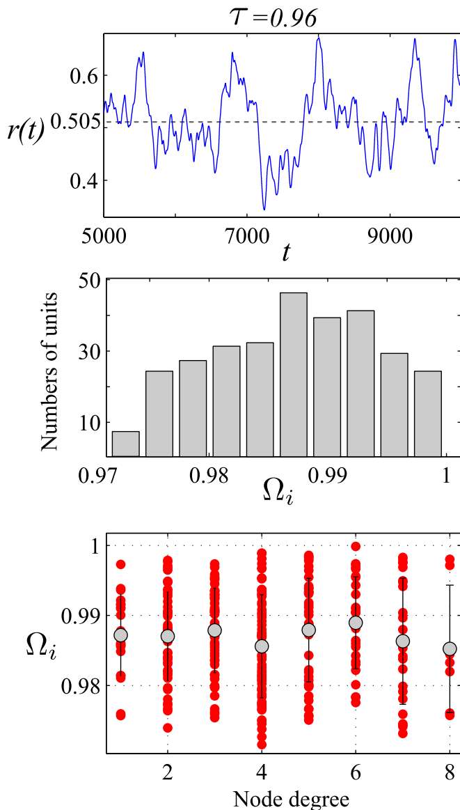
FIG. 5. Time evolution of the synchronization order parameter r(t) (top), histogram over the time averaged frequencies of all the oscillators (center), and frequencies versus node degree (bottom) for \tau = 0.96 . In this case the frequency distribution looks almost uniform and the order parameter fluctuates erratically. At this time delay, the time averaged order parameter r is equal to 0.505. The grey circles in the bottom figure marks the average frequency for each node degree. The result was obtained from a computer simulation of Eqs. (2) on a network with a binomial degree distribution with 300 nodes. The mean node degree \langle d_i \rangle was equal to 4, other parameters values were K = 0.1 , k = 4 and \omega = 1 .
