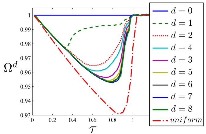
FIG. 2. Average frequency \Omega^d of all oscillators with degree d as a function of time delay on a network with binomial degree distribution. As can be seen, on average the nodes with lower degree loose connection with the larger cluster more quickly. The average frequency for the uniform network is also inserted in the figure as a reference. The network used in the simulation consisted of a total of 300 oscillators with mean node degree \langle d_i \rangle equal to 4. Other parameters values were K = 0.1 , k = 4 and \omega = 1 .
