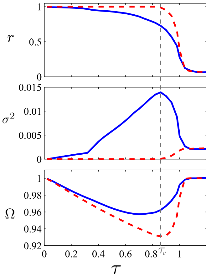
FIG. 1. Time averaged synchronization r , mean frequency dispersion \sigma^2 and mean frequency \Omega as a function of time delay \tau for a network of time delayed Kuramoto oscillators with identical degree distribution (dashed lines) and binomial degree distribution (solid lines). For each degree distribution, the values presented are averages taken from computer simulations of Eqs. (2) performed on 32 different networks each consisting of a total of 150 oscillators. In the case of an identical degree distribution we see an abrupt shift from synchronization to incoherence and negligible frequency dispersion. For the binomial degree distribution we see a more gradual shift from synchronization to incoherence accompanied by a pronounced frequency dispersion. The critical time delay \tau_c = 0.86 marks the beginning of the transition from synchronization to incoherence for the uniform network which happens to coincide with the maximum of the frequency dispersion for the non-uniform network. The mean node degree \langle d_i \rangle was equal to 4 in all cases, other parameters values were K = 0.1 , k = 4 and \omega = 1 .
