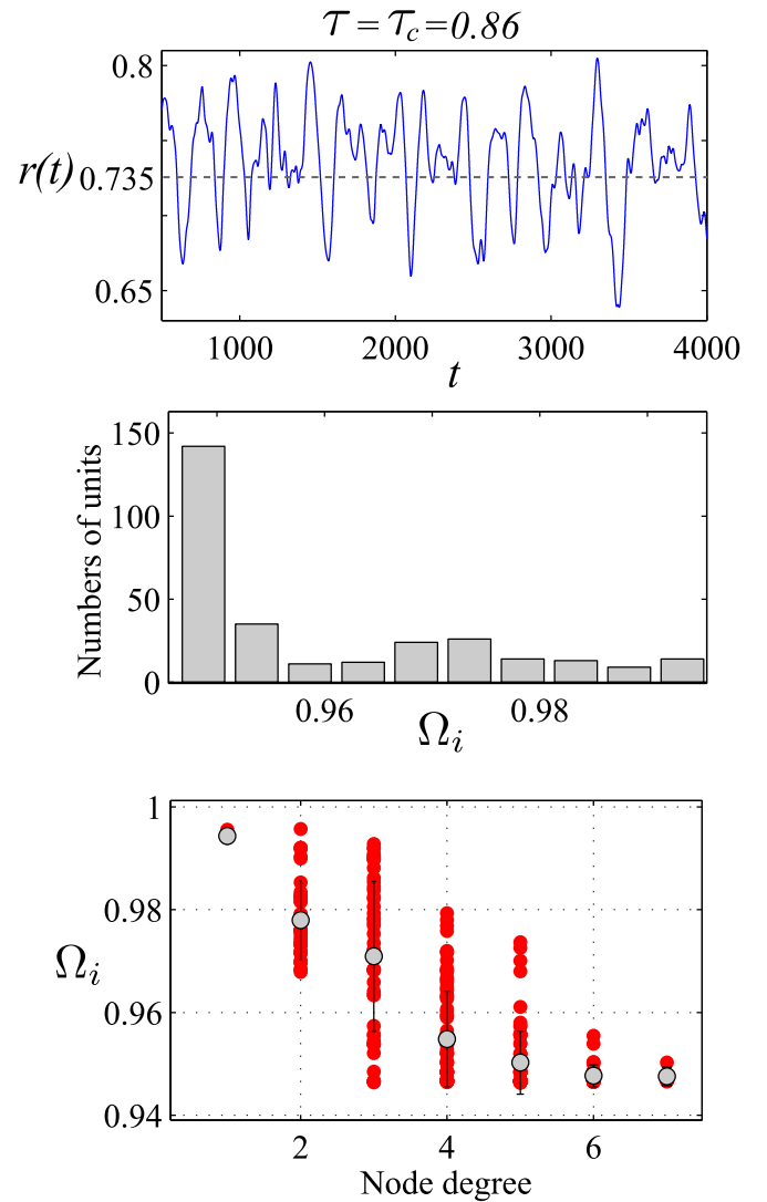
FIG. 4. Time evolution of the synchronization order parameter r(t) with root mean square r = 0.735 (top), histogram over the time averaged frequencies of all the oscillators (center), and frequencies versus node degree (bottom) for \tau = \tau_c = 0.86 . In this case approximately half of the oscillators are locked to a common frequency while the others are spread out. The grey circles in the bottom figure marks the average frequency for each node degree. The result was obtained from a computer simulation of Eqs. (2) on a network with a binomial degree distribution with 300 nodes. The mean node degree \langle d_i \rangle was equal to 4, other parameters values were K = 0.1 , k = 4 and \omega = 1 .
