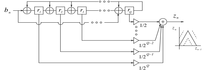
Fig. 3. Finite-state machine equivalent of an mTM CCM.
