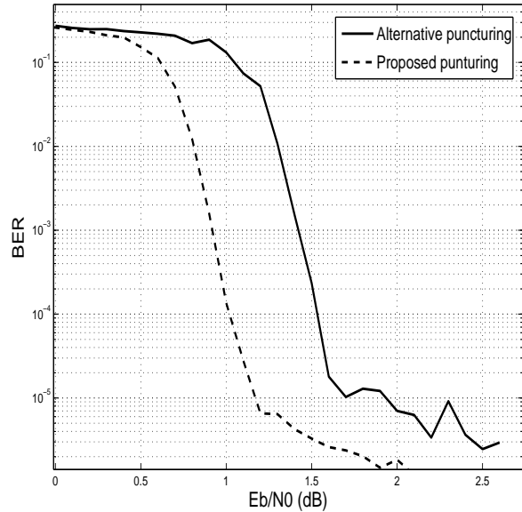
Fig. 8. Difference in the BER due to an alternative puncturing pattern.
