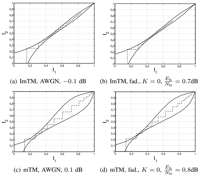
Fig. 13. EXIT charts vs. actual mutual information average trajectory for several PCCCM cases and environments. In all the cases, we use phase mapping, no puncturing, the quantization factor is Q = 5 , and the interleaver chosen for the mutual information evolution simulations is an S-random interleaver with N = 5500 ans S = 19 .
