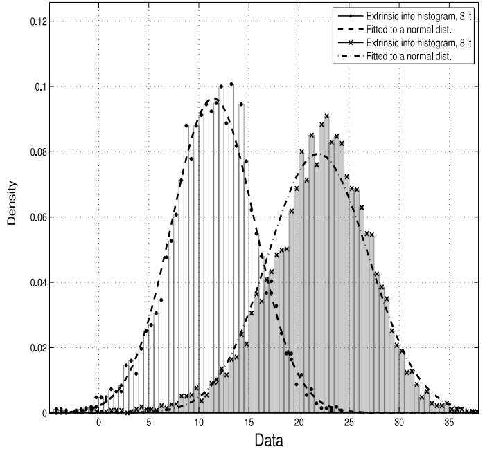
Fig. 12. Histogram of the extrinsic data for an ImTM PCCCM, after 3 and 8 decoding iterations, for E_b/N_0=1 dB.
