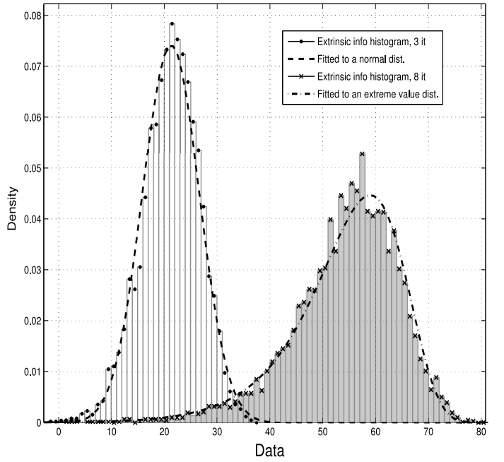
Fig. 11. Histogram of the extrinsic data for a mTM PCCCM, after 3 and 8 decoding iterations, for E_b/N_0=1 dB.
