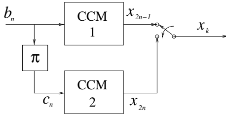
Fig. 1. Scheme of the unpunctured concatenated coded modulator.
