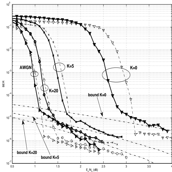
Fig. 17. BER results in the flat fading channel for different values of K . TTCM (dashed line) is compared with the ImTM/ImTM punctured PCCCM system (solid boldline) of same spectral efficiency. Bounds are depicted in dash-dotted line.
