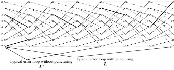
Fig. 10. Trellis of a Bernoulli shift map based CCM with Q = 3 . Solid: transition triggered by a 0. Dotted: transition triggered by a 1. Strong boldline: path through the trellis followed by a typical error event. Weak boldline: punctured out symbol and transition.
