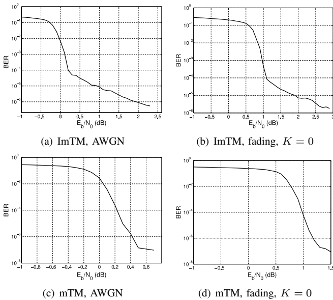
Fig. 14. BER simulations corresponding to the cases depicted in Fig. 13.
