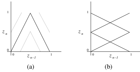
Fig. 5. Maps for the main constituent CCM encoders. (a) mTM; (b) ImTM.
