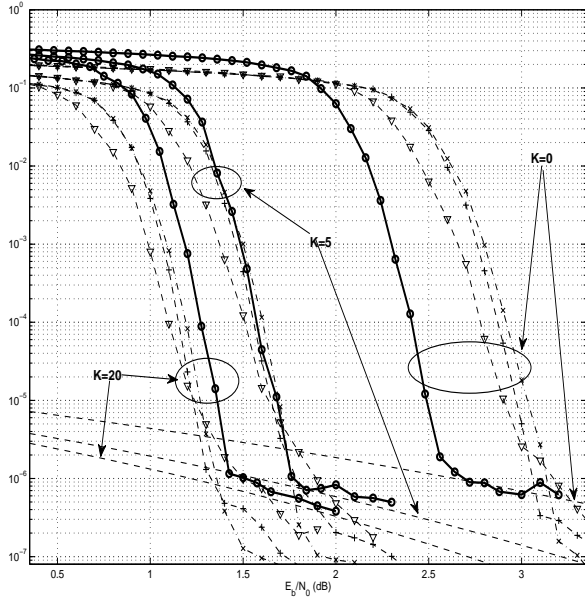
Fig. 15. Results in the Rician flat fading channel for different values of K . CDMA2000 turbocode is depicted in dashed line, '+', UMTS turbocode is depicted in dash-dotted line, 'x', and WiMAX duobinary turbocode is depicted in dashed line, 'v'. ImTM/mTM PCCCM results are depicted in solid line, 'o'.
