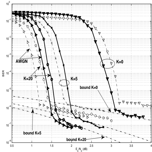
Fig. 18. BER results in the flat fading channel for different values of K . TTCM (dashed line) is compared with the ImTM/mTM punctured PCCCM system (solid boldline) of same spectral efficiency. Bounds are depicted in dash-dotted line.
