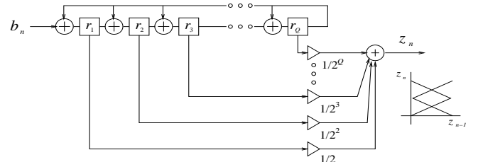
Fig. 4. Finite-state machine equivalent of an ImTM CCM.
