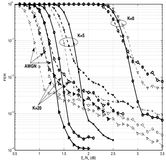
Fig. 19. FER results in the flat fading channel for different values of K . TTCM results (dashed thin line) are compared with ImTM/ImTM punctured PCCCM system results (dashed boldline), and with ImTM/mTM punctured PCCCM system results (solid boldline).
