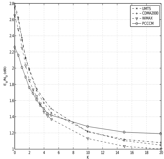
Fig. 16. E_b/N_0 (dB) needed to reach a BER of 10^{-3} for different values of K , ranging from 0 to 20.
